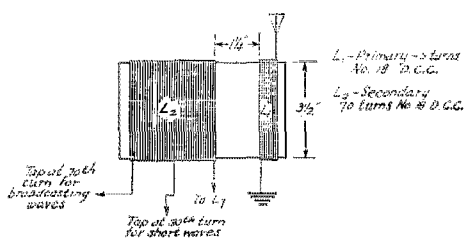
Transformer details, see Fig. 6 for connections of complete set. FIG. 4B
