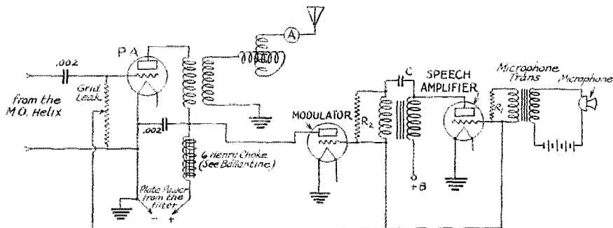
FIG. 5 COMPLETE MODULATION CIRCUIT (shown here for the series-feed P.A. of Fig. 3 but can be used with many other circuits) The right sizes for R_1 , R_2 and C must be found by trial.
