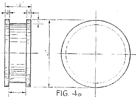
SPOOL FOR TUNED CHOKE WINDING 200 TURNS NO. 24 D.S.C. "SCRAMBLE WOUND"
